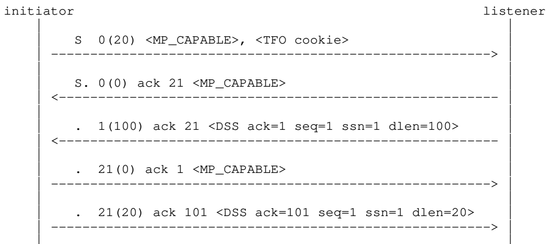
Figure 19: The Listener Supports TFO
