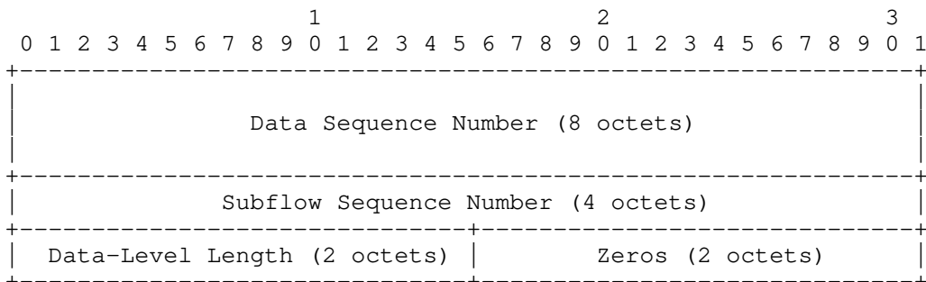
Figure 10: Pseudo-Header for DSS Checksum
