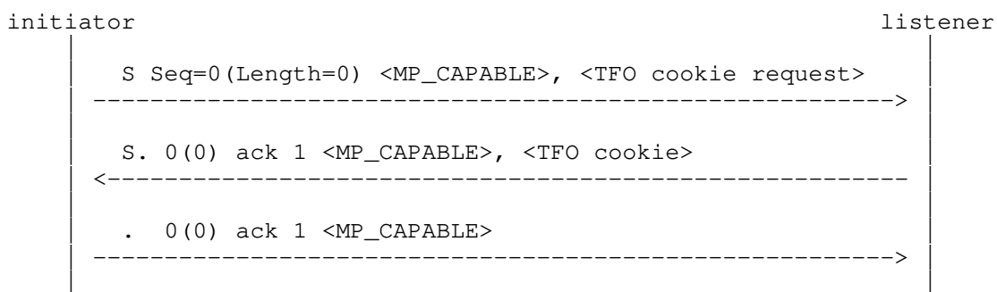
Figure 18: Cookie Request
