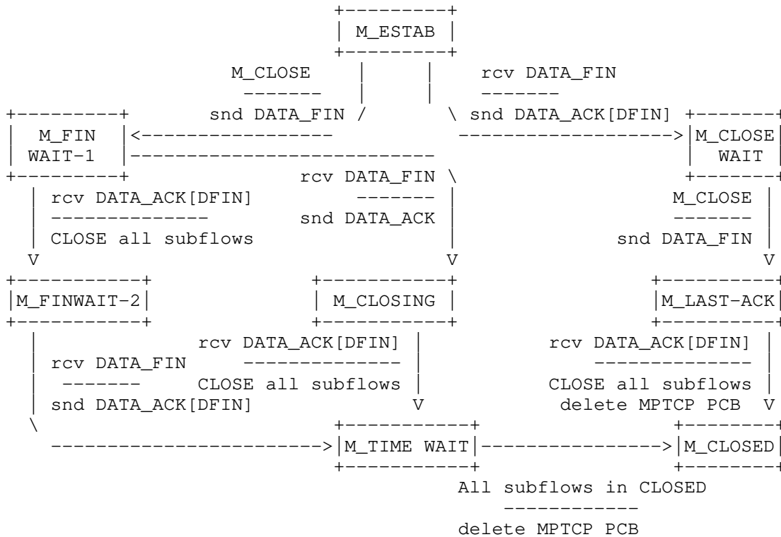
Figure 22: Finite State Machine for Connection Closure
