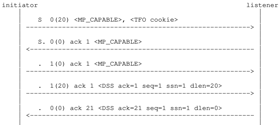
Figure 20: The Listener Does Not Support TFO
