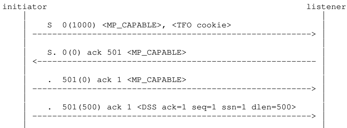
Figure 21: Partial Data Acknowledgment
