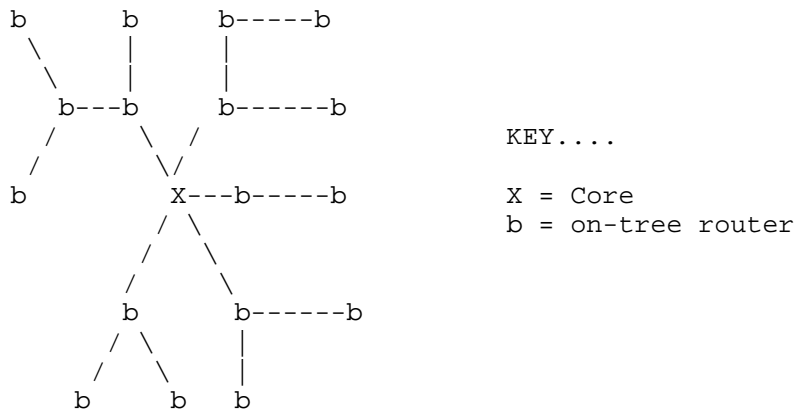
Figure 2: CBT Tree
